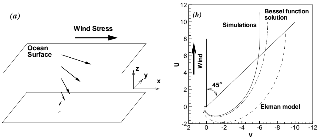
FIGURE 1. (a), Model geometry. (b), Time- and horizontally averaged hodographs of the horizontal current. —, calculations at 90°-latitude, ---, Ekman profile (1.1), - · - · - ·, Bessel function solution (3.8) obtained with a piecewise-linear effective viscosity profile (see section 3.3 for details).
