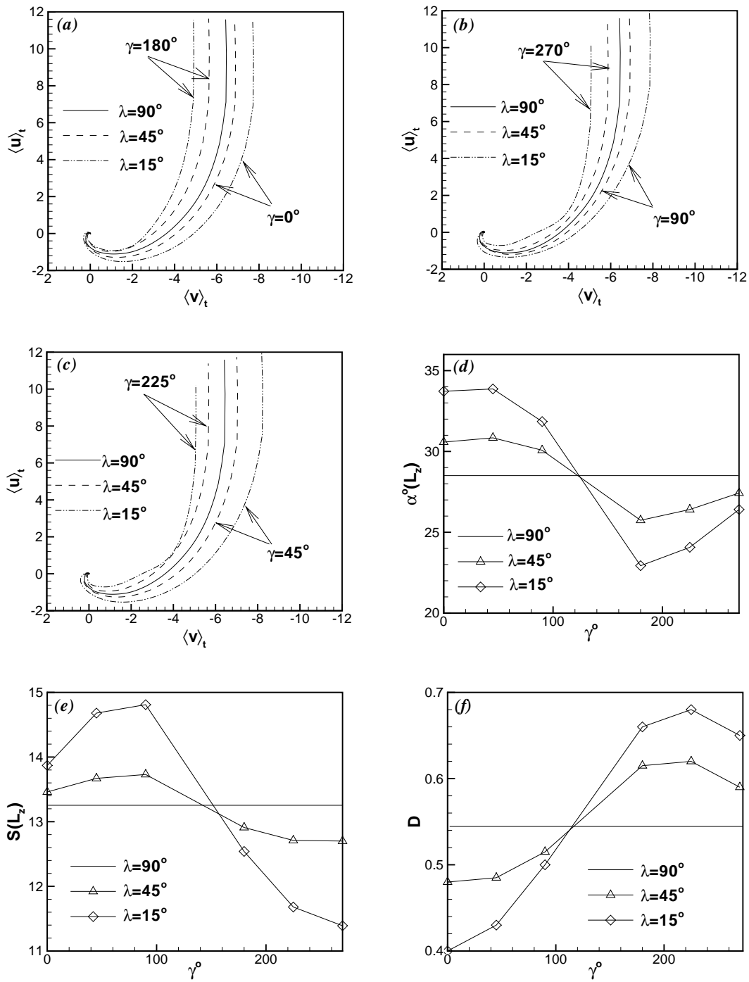
FIGURE 7. Impact of latitude \lambda and the wind angle \gamma on the mean velocity profile. (a)-(c), velocity hodographs; (d), surface angle \alpha(L_z) between the current and the wind direction as a function of \gamma at different \lambda ; (e), speed of the surface current S(L_z) ; (f), depth of exponential decay of the current D .
