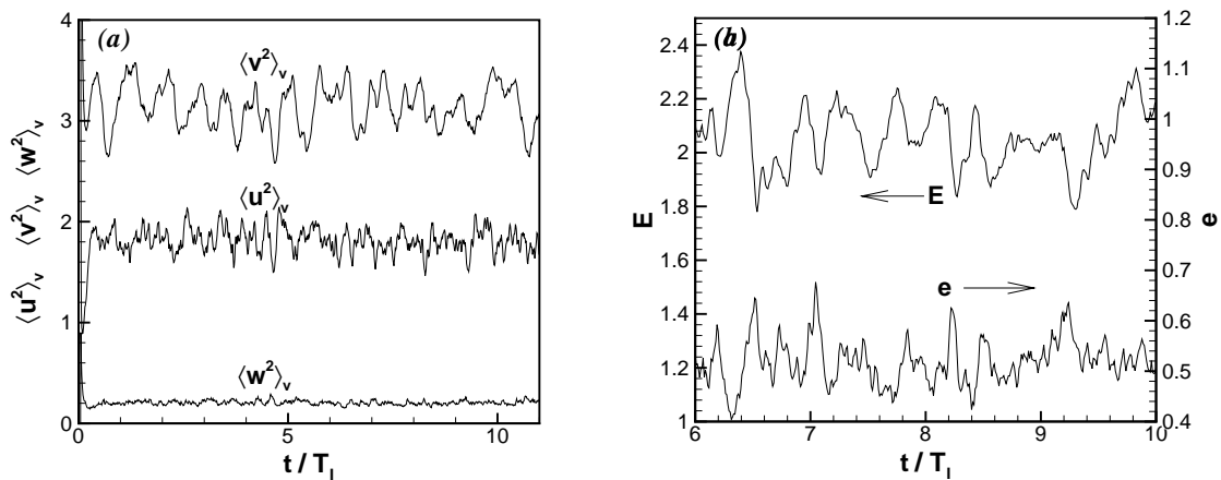
FIGURE 2. Volume-averaged kinetic energy as a function of time at the latitude 90^\circ . (a), Energy of each velocity component, \langle u^2 \rangle_v , \langle v^2 \rangle_v , and \langle w^2 \rangle_v . (b), Kinetic energy of the mean horizontal current ( E ) and turbulent fluctuations ( e ).
