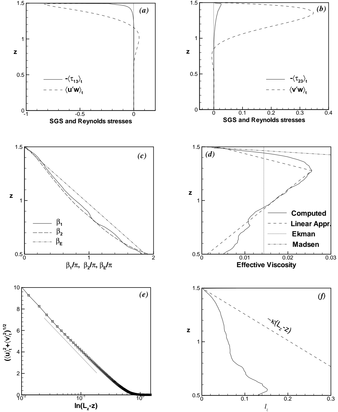
FIGURE 5. Horizontally and time-averaged profiles calculated in the developed turbulent flow at 90^\circ -latitude. (a), x - z components of subgrid-scale and Reynolds stresses; (b), y - z components of subgrid-scale and Reynolds stresses; (c), Angles between the wind direction and, correspondingly, the direction of the total stress vector ( \beta_1 ), mean shear vector ( \beta_2 ), and the shear vector in the Ekman solution ( \beta_E ); (d), —, Effective viscosity coefficient (3.5) evaluated using the computed stress and shear profiles, - · - · - ·, linear dependence A_z = \kappa(L_z - z) used by Madsen (1977); · · · · ·, constant viscosity coefficient A_{zE} = 0.0144 of the Ekman model, - - -, Piecewise-linear approximation of the viscosity profile used for an approximate solution (3.8); (e), Amplitude of the mean current vs. logarithm of depth; (f), Mixing length (3.6).
