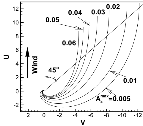
FIGURE 10. Velocity hodographs obtained as the Bessel function solutions (3.8) for z_{max} = L_z - 0.222 and varying
