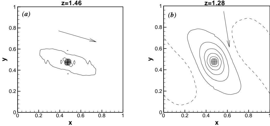
FIGURE 3. Two-point velocity correlations (C_{11} + C_{22} + C_{33})/3 (see (3.1)) in the developed turbulent flow at 90^\circ -latitude. The correlations are calculated at (a) z = L_z - 0.04 and at (b) z = L_z - 0.22 and averaged over the time period of 5T_I . Contour step is 0.1. The contour levels range between 0.05 and 0.95 in (a), and between -0.05 (shown by dashed lines) and 0.95 in (b). Arrows show the direction of the time-averaged mean shear d(\langle u \rangle_t, \langle v \rangle_t)/dz .
