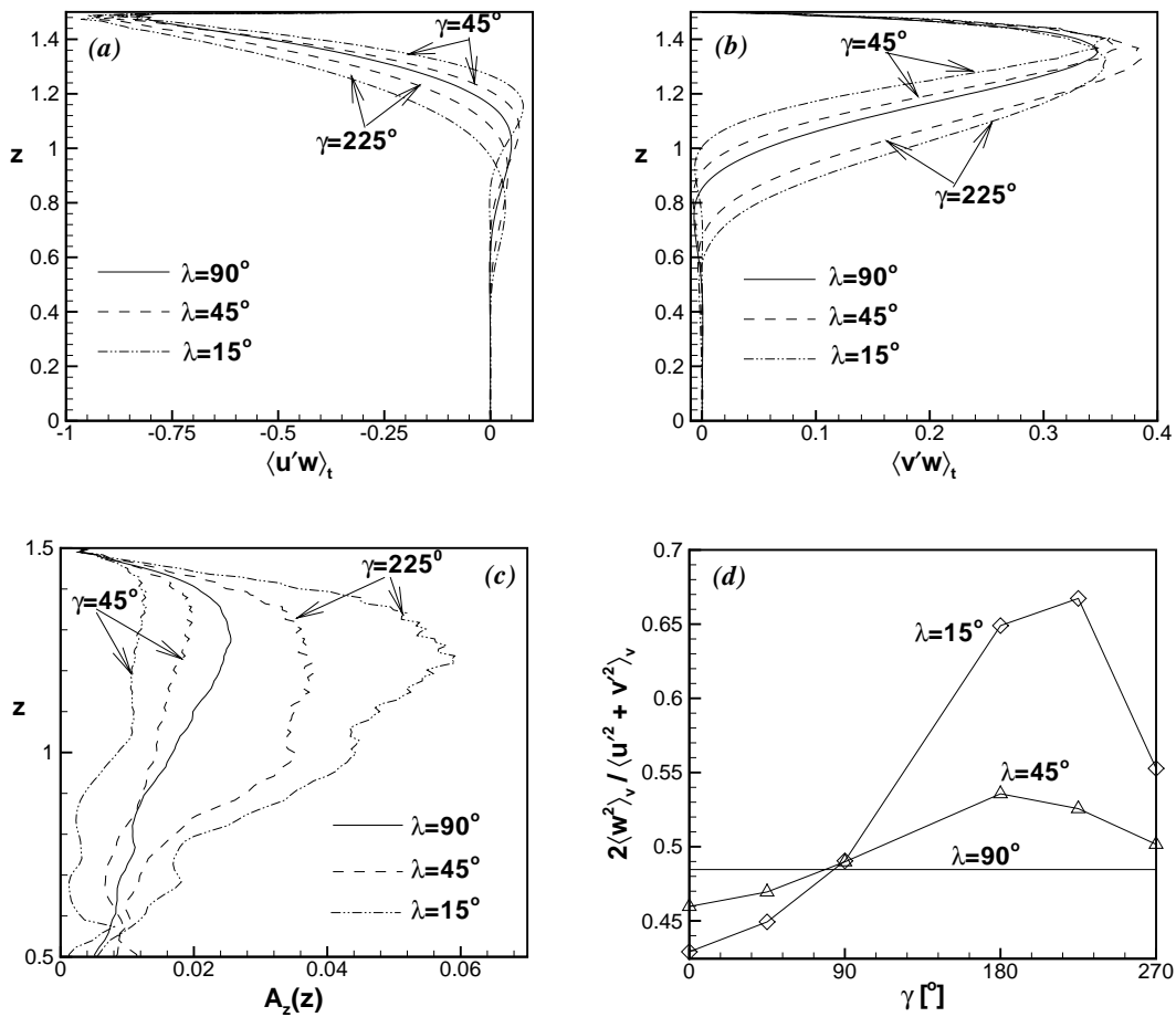
FIGURE 8. Effect of the latitude \lambda and wind angle \gamma on the properties of turbulent fluctuations. (a), x - component \langle u'w \rangle of the turbulent momentum transfer; (b), y - component \langle v'w \rangle of the turbulent momentum transfer; (c), Effective viscosity A_z(z) . (d), Ratio 2\langle w^2 \rangle_v / \langle u'^2 + v'^2 \rangle_v between the volume- and time-averaged turbulent kinetic energy of vertical and horizontal velocity fluctuations.
