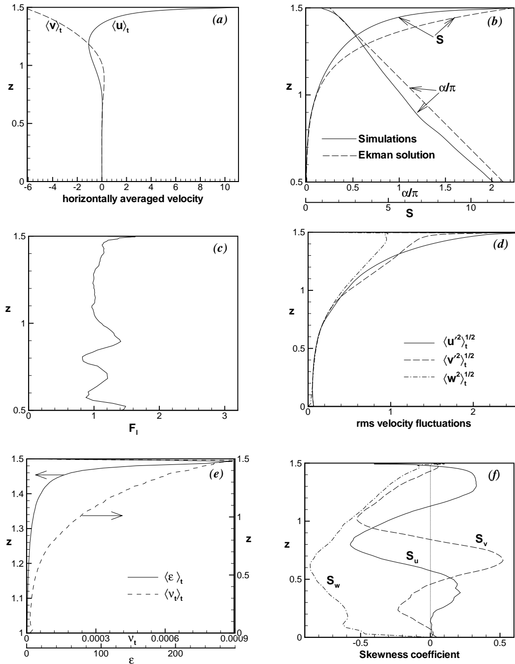
FIGURE 4. Horizontally and time-averaged profiles calculated in the developed turbulent flow at 90^\circ -latitude. (a), Components of the mean horizontal current \langle u \rangle_t and \langle v \rangle_t ; (b), Angle \alpha between (\langle u \rangle_t, \langle v \rangle_t) and the wind direction and the speed of current S ; (c), Flatness coefficient F_l (3.2); (d), Root-mean-square velocity fluctuations; (e), Mean turbulent eddy viscosity \nu_t (2.14) and the rate of subgrid-scale kinetic energy dissipation \epsilon_t (3.3) (note different vertical and horizontal scales used to plot \nu_t and \epsilon_t ); (f), Skewness coefficients (3.4) of the velocity components.
