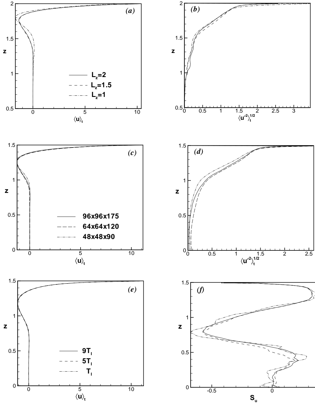
FIGURE 12. Verification of the accuracy of the numerical model. Horizontally and time-averaged profiles calculated in the developed turbulent flow at 90^\circ -latitude. (a) and (b), mean velocity and rms perturbations calculated in the domains with different vertical size; (c) and (d), mean velocity and rms perturbations calculated with different numerical resolution; (e) and (f), profiles of mean velocity and skewness coefficient obtained by averaging over different time intervals.
