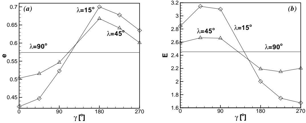
FIGURE 9. Effect of the latitude \lambda and wind angle \gamma on the flow energy. (a), energy of turbulent fluctuations
