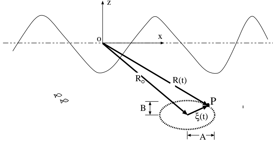
Particle trajectory in a progressive wave.
